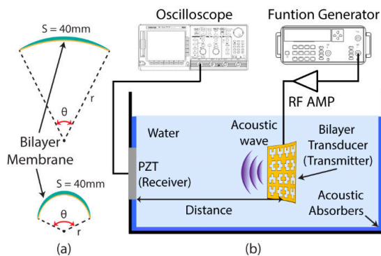
Fig. 4. An experimental setup for (a) mimicked deformed bilayer transducer in (b) a water tank.
