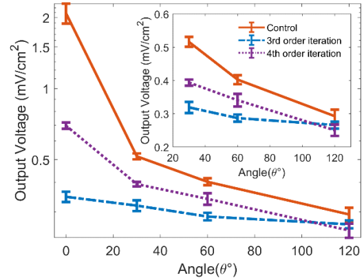
Fig. 7. Wirelessly received voltage due to various curved bilayer transducers (indicating pH).
