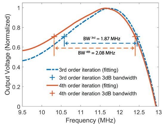
Fig. 6. Frequency response.
