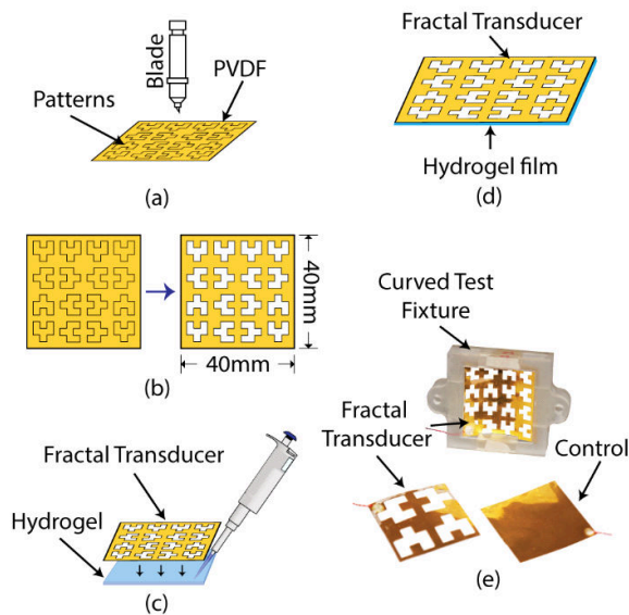
Fig. 3. Fabrication: (a), (b) modified Hilbert curve is carved out from PVDF thin film, (c) lay out the PVDF film on hydrogel, (d) cure hydrogel and complete a transducer; (e) prototypes.
