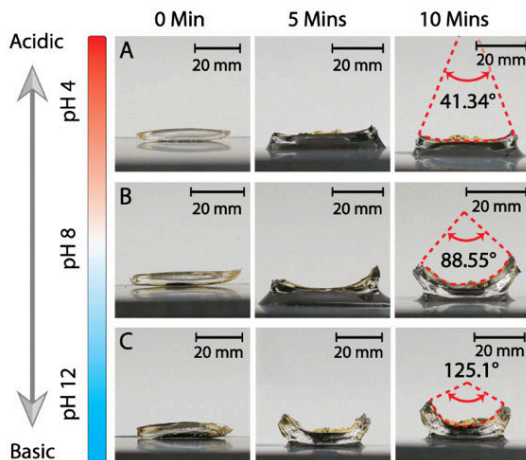
Fig. 5. pH responsive curvatures.
