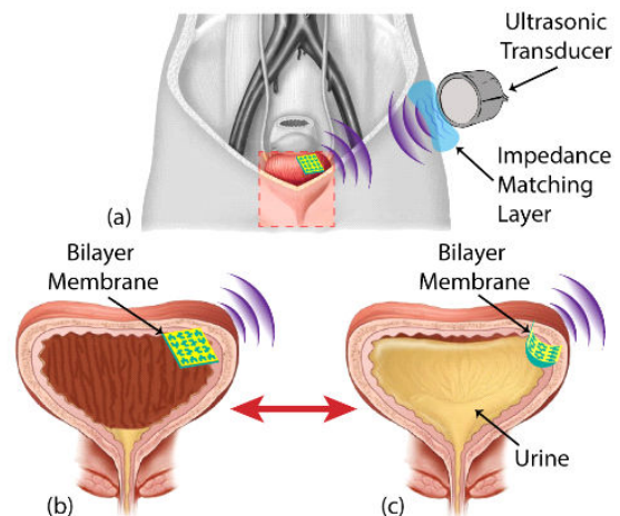
Fig. 1. (a) Schematic view of the proposed hydrogel-fractal bilayer transducer for wireless pH sensing; (b), (c) urine induce curvature in the transducer, resulting in resonant frequency shift.
