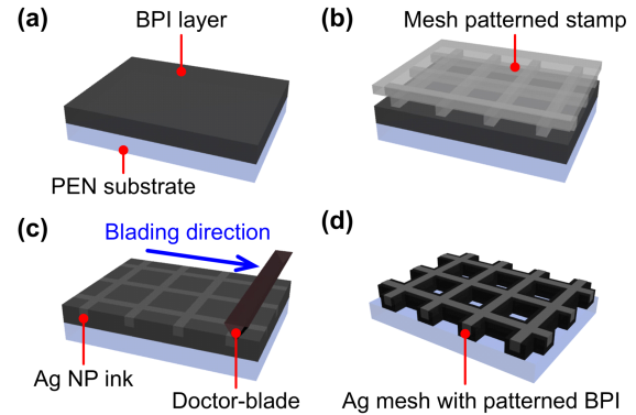
Fig. 1. Fabrication process of Ag metal mesh electrodes with a patterned BPI light absorption layer. (a) Bar-coated BPI layer on a PEN substrate. (b) Thermal imprinting of recessed mesh channels using a mesh-patterned PDMS stamp. (c) Doctor-blade filling of Ag NP ink after UVO treatment; the arrow indicates the blading direction. (d) Ag metal mesh electrode with patterned BPI after thermal treatment and selective etching.
