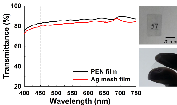
Fig. 4. Optical transmittance of the Ag metal mesh electrode film. Transmittance spectra of the bare PEN film and Ag metal mesh electrode film, with photographs showing the transparency and flexibility of the fabricated sample.
