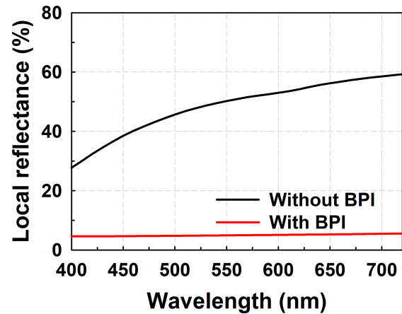
Fig. 3. Local reflectance of the Ag electrode region. Reflectance spectra without BPI (black line) and with BPI (red line), showing reduced local reflectance after BPI integration.
